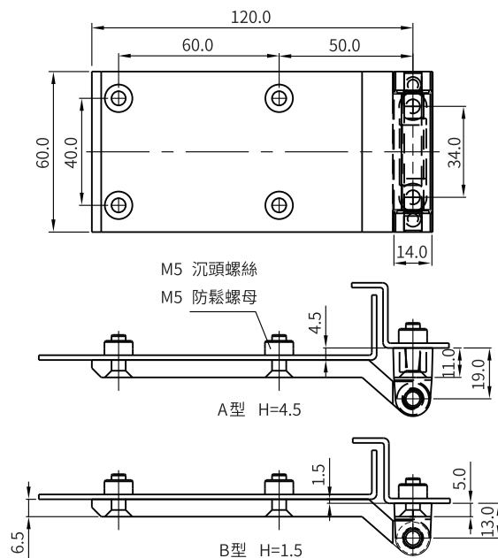
鉅合金螺絲固定鉸鏈,不鏽鋼銷軸,PA襯套 Screw-oc hinge zinc die, pin stainless steel and bushes polyamide
