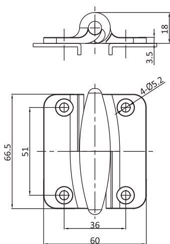
L型 (左裝) Version L(Left) B-2115-76604-L
