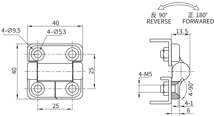
M5沉頭螺絲固定 Countersunk Screw M5
