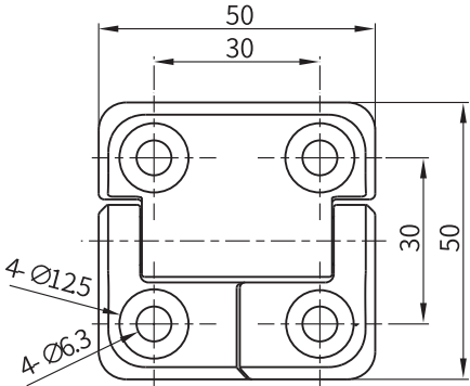
M6沉頭螺絲固定 Countersunk Screw M6
