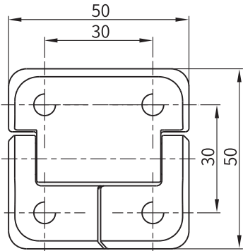
M6鑲嵌螺柱 With Threaded Studs M6
