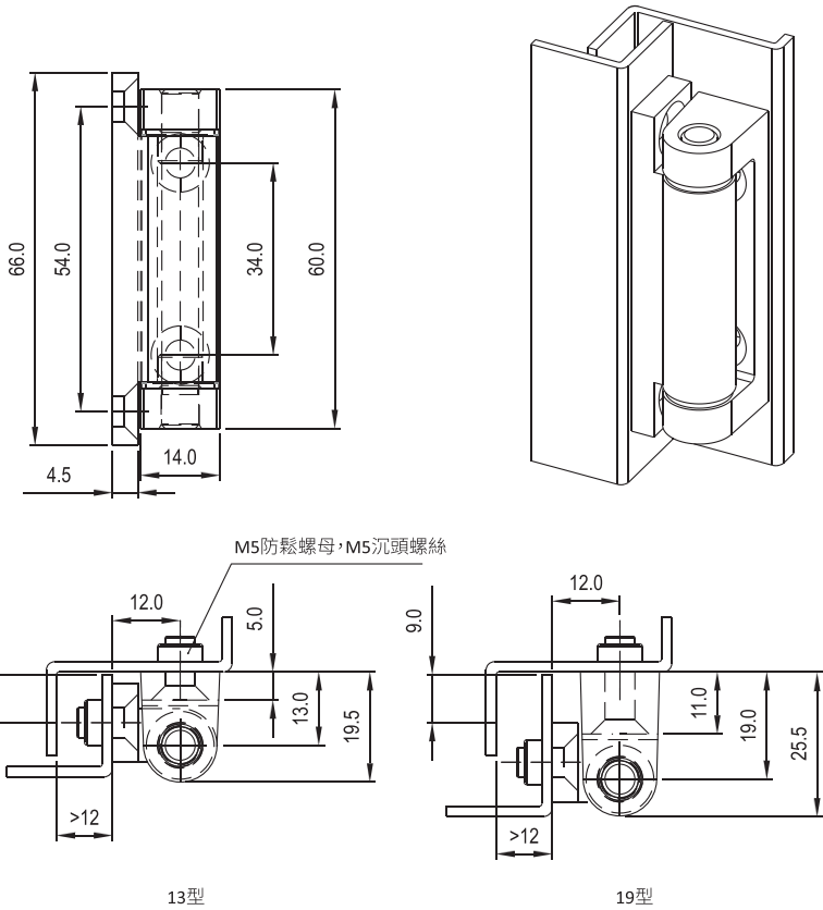
鋅合金鉸鏈, 不鏽鋼銷軸和PA襯套 Hinge zinc die, m.s.zinc plated pin, PA bousing
