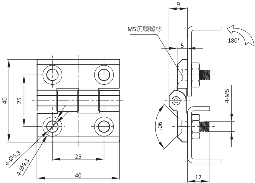
M5 沉頭螺絲固定 Countersunk Screw M5
