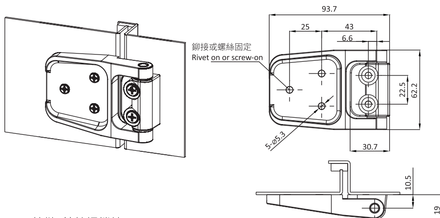
黑色PA+GF鉸鏈, 鍍鋅鋼銷軸 Hinge Polyimide GF 30% black, M.S. zinc plated pin
